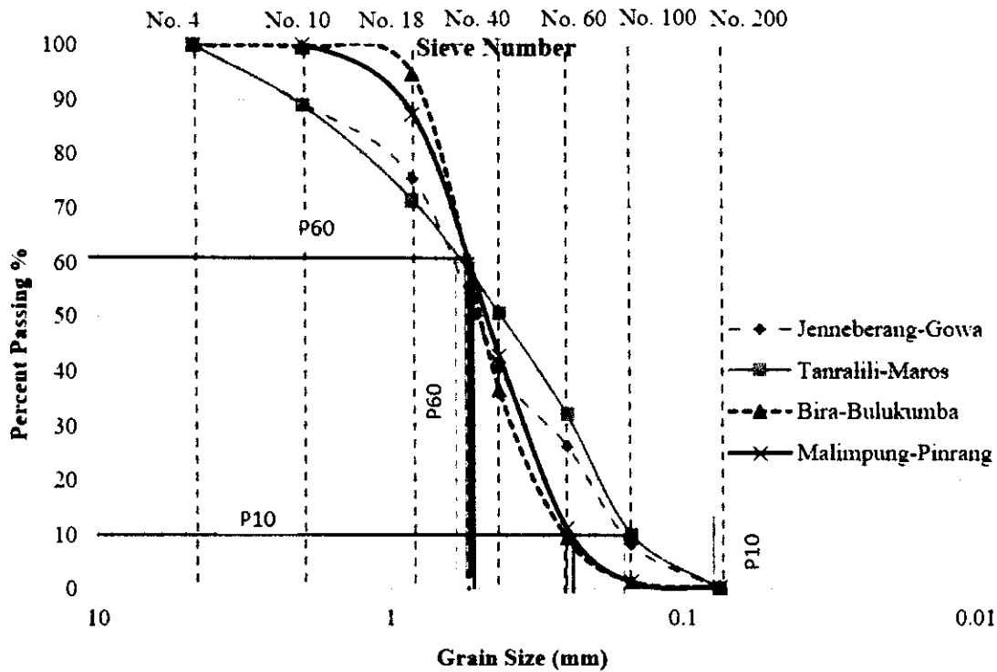
Fig. 3 Sieve analysis results
