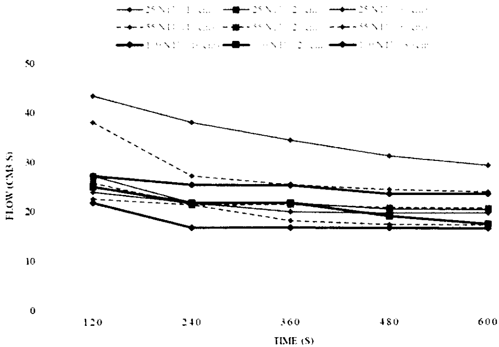
Fig. 7 The effect of time on changes of discharge in the Malimpung-Pinrang sand
