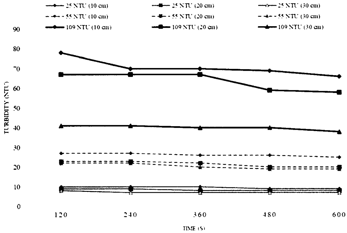
Fig. 6 The effect of time on the decrease in the NTU of Malimpung-Pinrang sand
