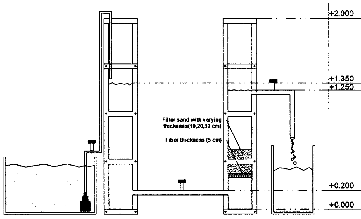
Fig. 1 The simulation equipment of the filtration process
